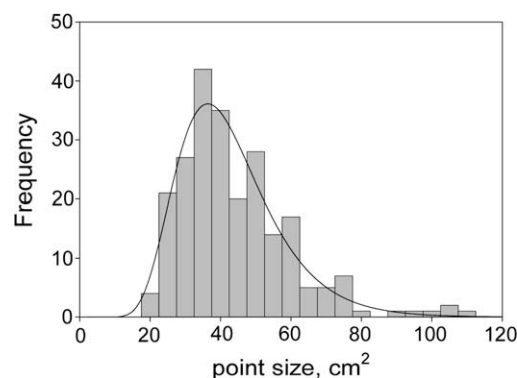
Fig. 5. Frequency distribution of the projectile point sizes ( n = 232 ). The distribution is skewed to the right and well-fit by a lognormal distribution, as predicted (solid line).
